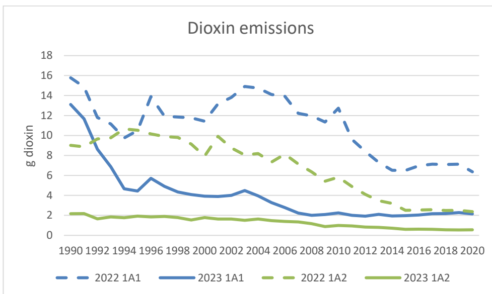
Figure XX. Effects of revision of Dioxin between submission 2022 and 2023 in NFR 1A1 and 1A2.
