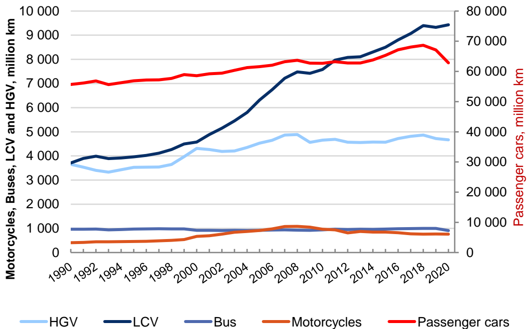
Figure A2-11. Vehicle mileages 1990-2021 according to HBEFA 4.2.
