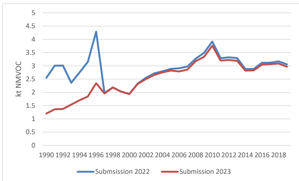
Figure XX. Effects of revision of NMVOC between submission 2022 and 2023 in NFR 1A1a.
