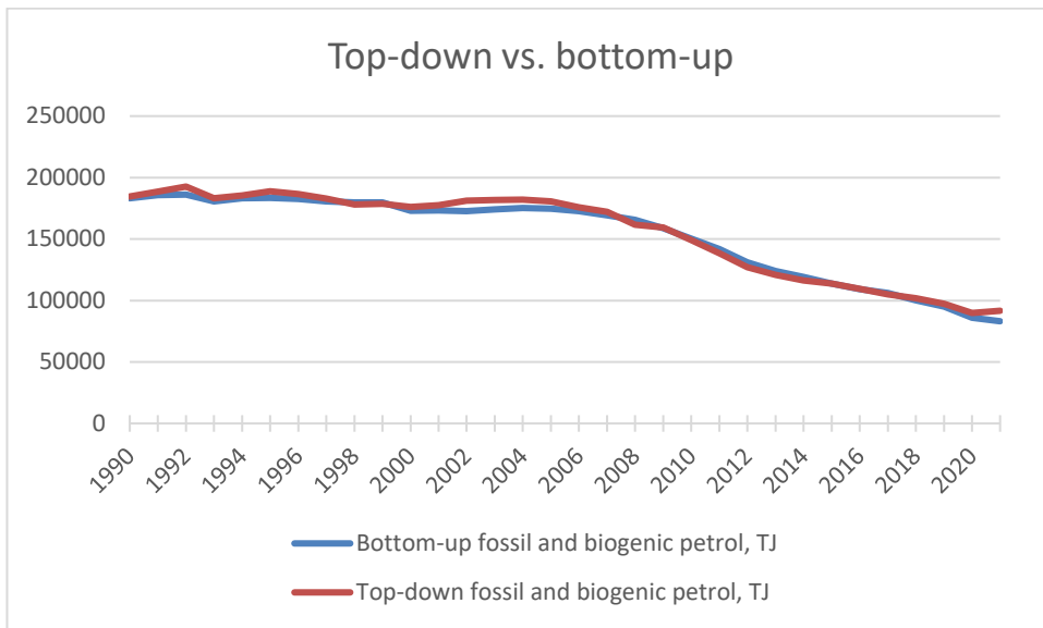
Figure A2-2. Bottom-up vs. top-down approach for petrol in submission 2023.
